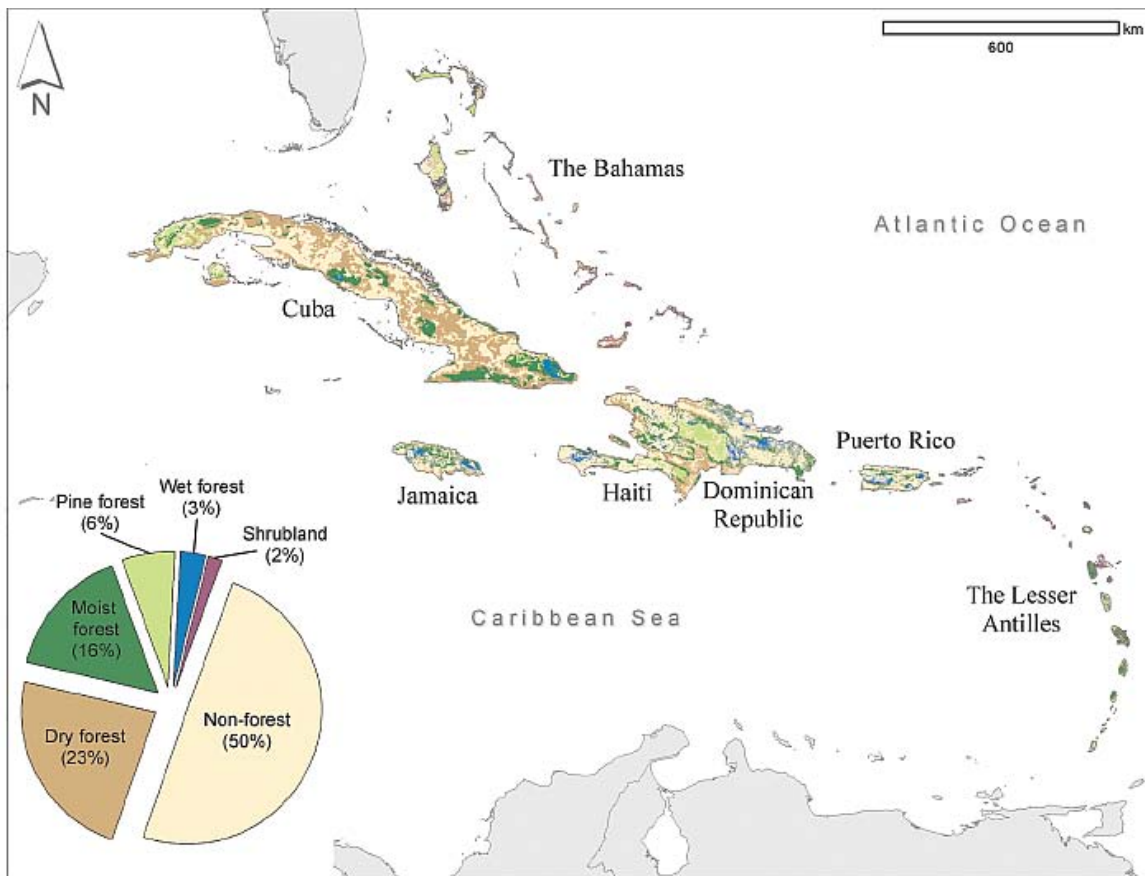
Figure 2. Simplified vegetation map of the insular Caribbean. Spatial data were modified from Huggins et al. (16).
